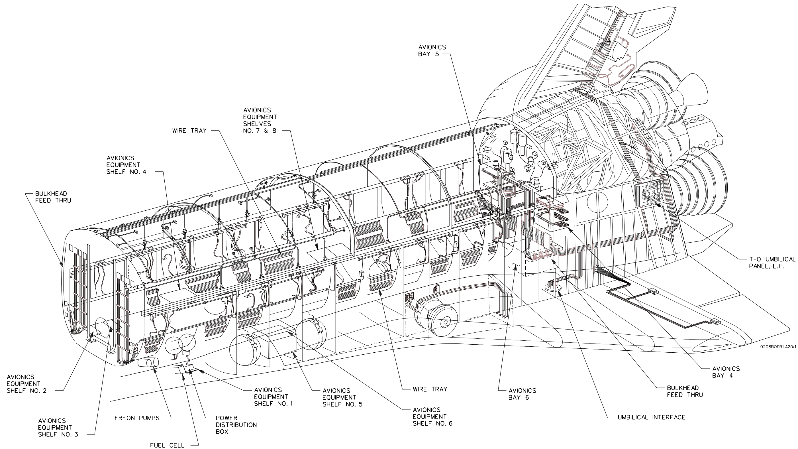
(b) Mid- and aft fuselage.
