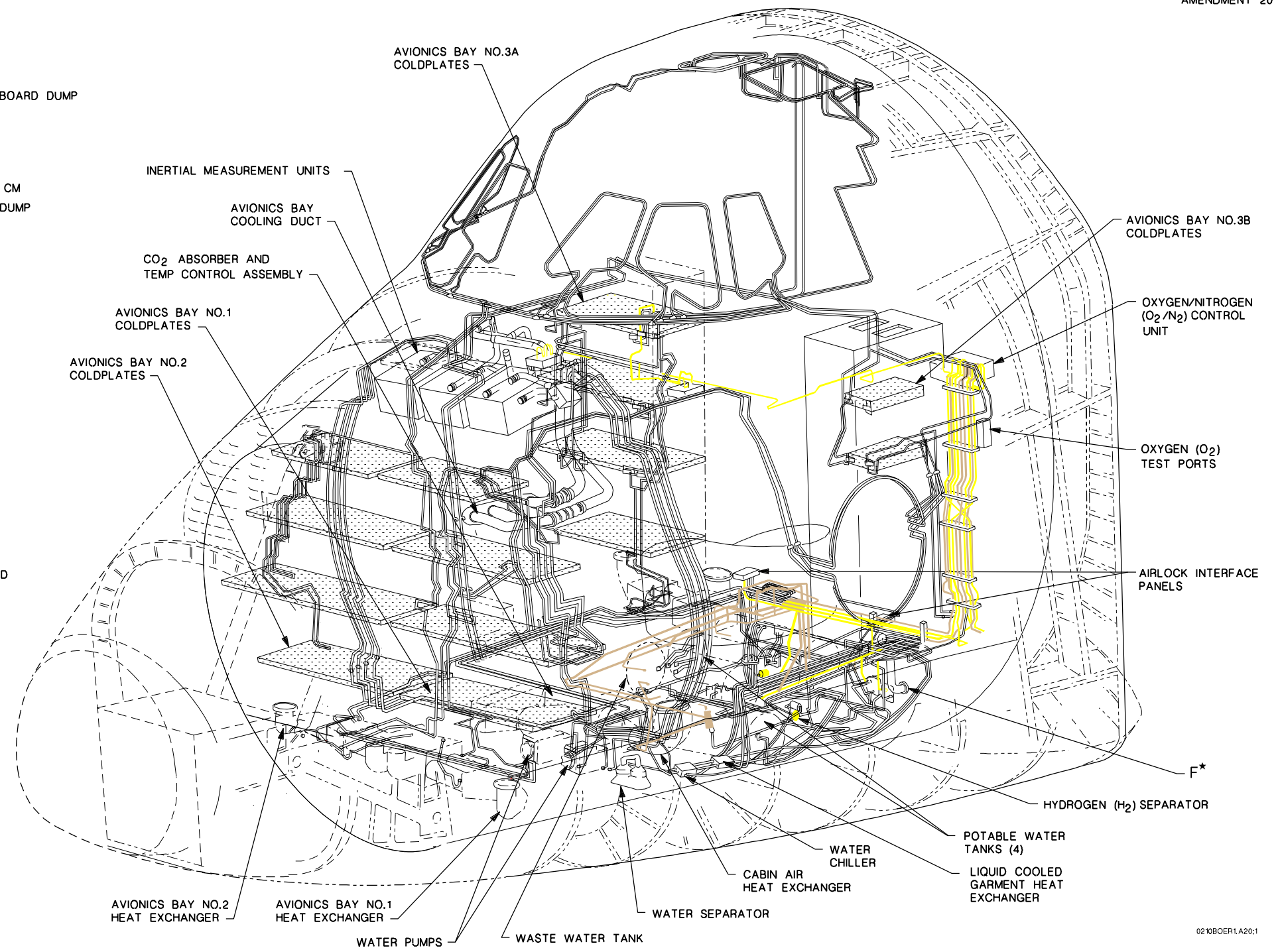
(b) Forward fuselage coolant/air revitalization components.
