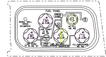
FUEL PANEL
