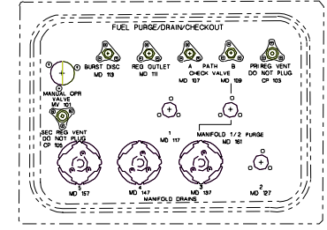
FUEL PURGE/DRAIN/CHECKOUT
